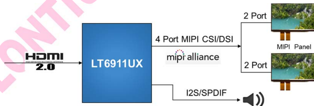
Figure1. Application Diagram
